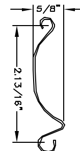
24 GAUGE CURVED SLAT
