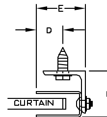
U-GUIDE FOR STEEL/WOOD
