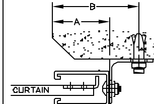
WINDLOCK FOR CONCRETE OR MASONRY
