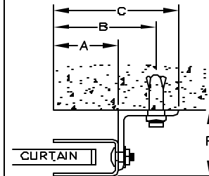
Z-GUIDE FOR CONCRETE/MASONRY
