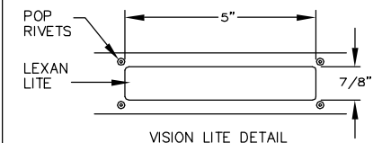
VISION LITE DETAIL
