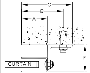
Z-GUIDE FOR CONCRETE/MASONRY
