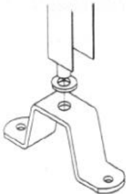
PEDESTAL MOUNT INSTALLED HEIGHT MATCHES CASTER HEIGHT
